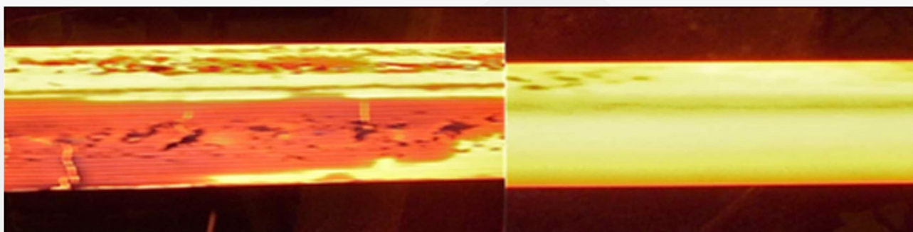
Fig. 11 Billet WAVE marks visible when entering the mill but gone after second pass
